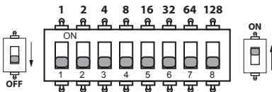
Delay Time Period Setting Switch 3
