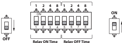
Pulsing Time Period Setting Switch 3
